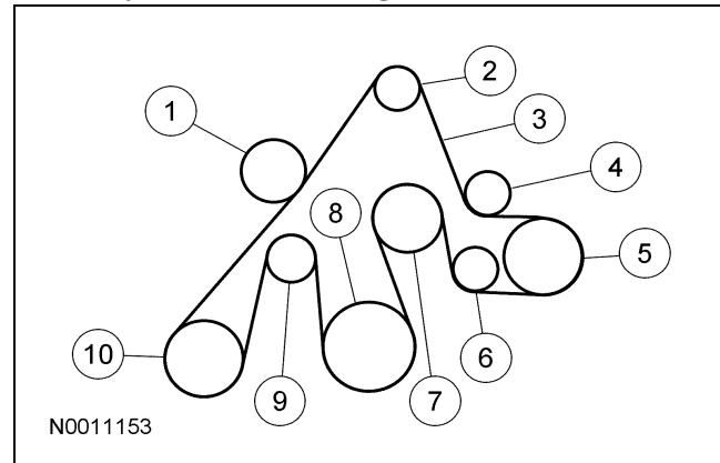
Accessory Drive Belt Routing — 4.6L (3V)
