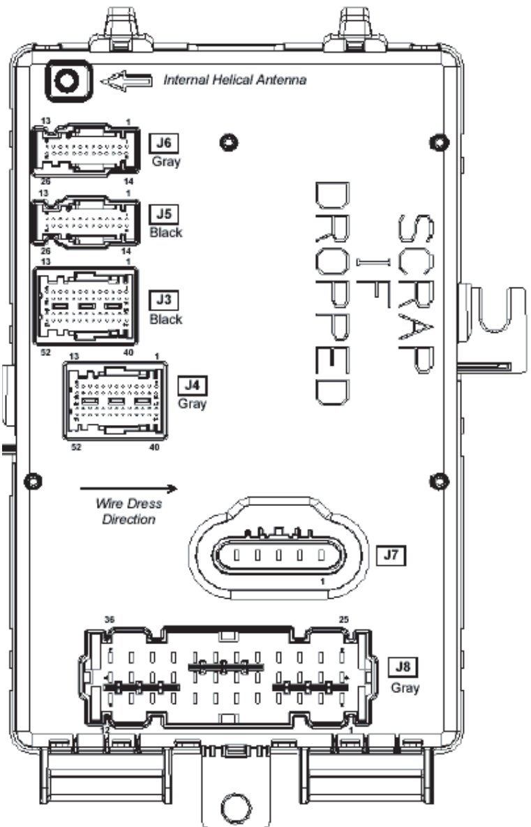
S197 SJB Layout (Back View)
